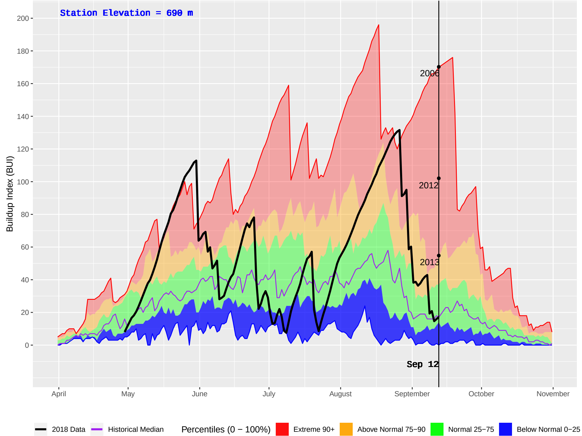
MACKENZIE FS (155) : Historical (1994–2016) and Current (2018) Daily Buildup Index (BUI)
